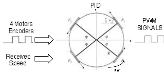
Fig. 8 Motor control using Pulse Width Modulation (PWM) and Proportional-Integral-Derivative controller (PID).
